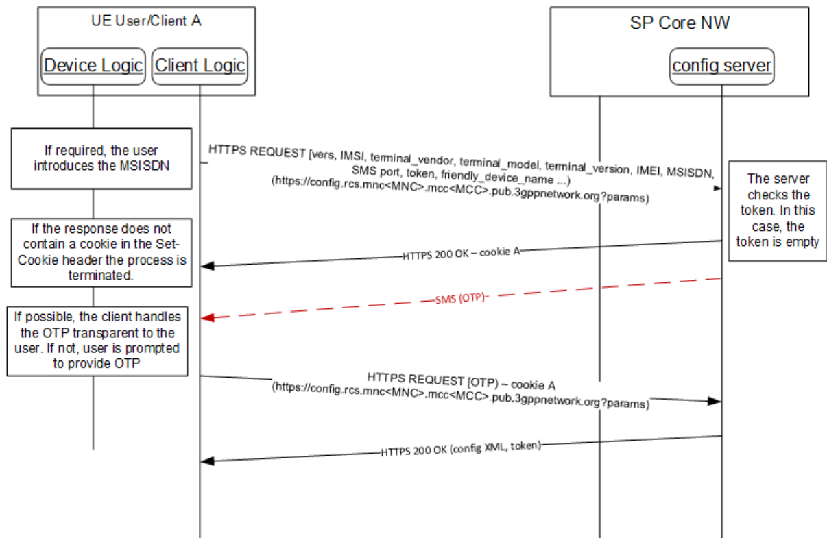
Figure 3: HTTP configuration for primary devices over non-PS access with MSISDN: empty token
